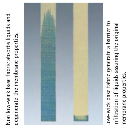
Comparison between low-wick and non low-wick base fabric
