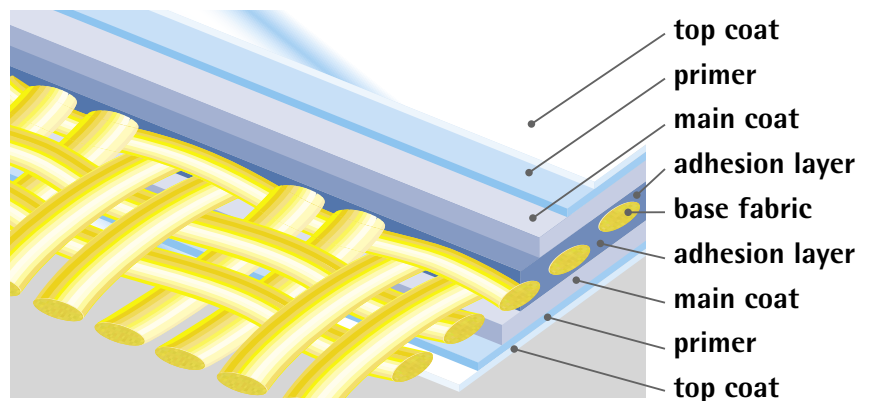
Typical section of Mehler coated PVC-Polyester fabric
